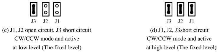
Figure 2: J1 and J3 jumpers
