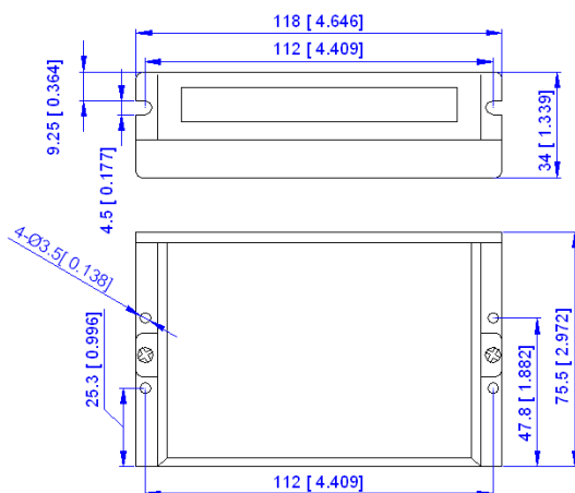
Figure 1: Mechanical specifications
